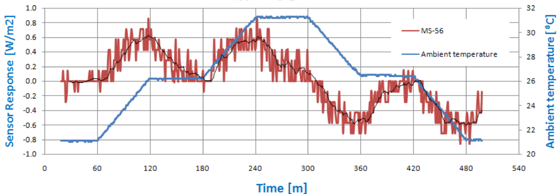
Figure 7-3. Zero Offset Measurement
