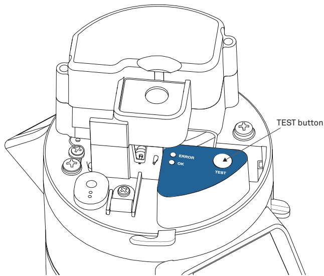
Figure 28 TEST button
