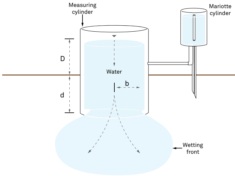
Figure 29 Cross section of a single-ring infiltrometer
