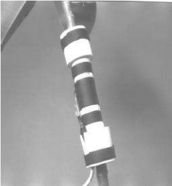
Figure 4.6 - O-rings installed
