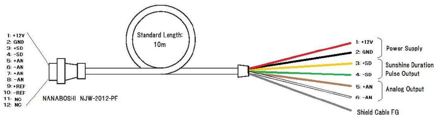
Figure 8-1.Sensor Output Cable
