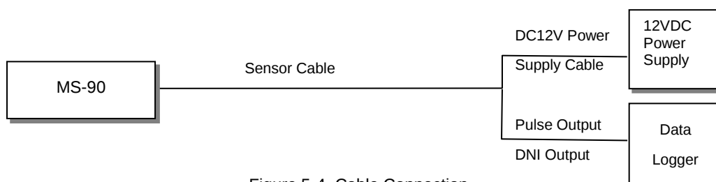
Figure 5-4. Cable Connection
