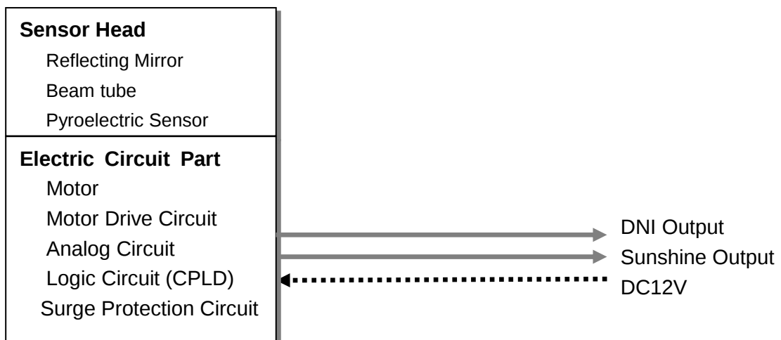
Figure 5-2. Configuration
